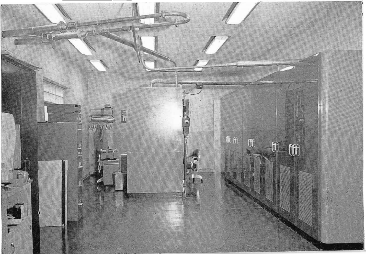
FIG. 3. Above floor plan shows arrangement of TV transmitter and studio facilities. Plans call for expansion of TV building to include new TV studios and WDAF AM studios. Below is a rear view of the TT-5A, with vestigial sideband filter (center) and diplexer mounted overhead.
