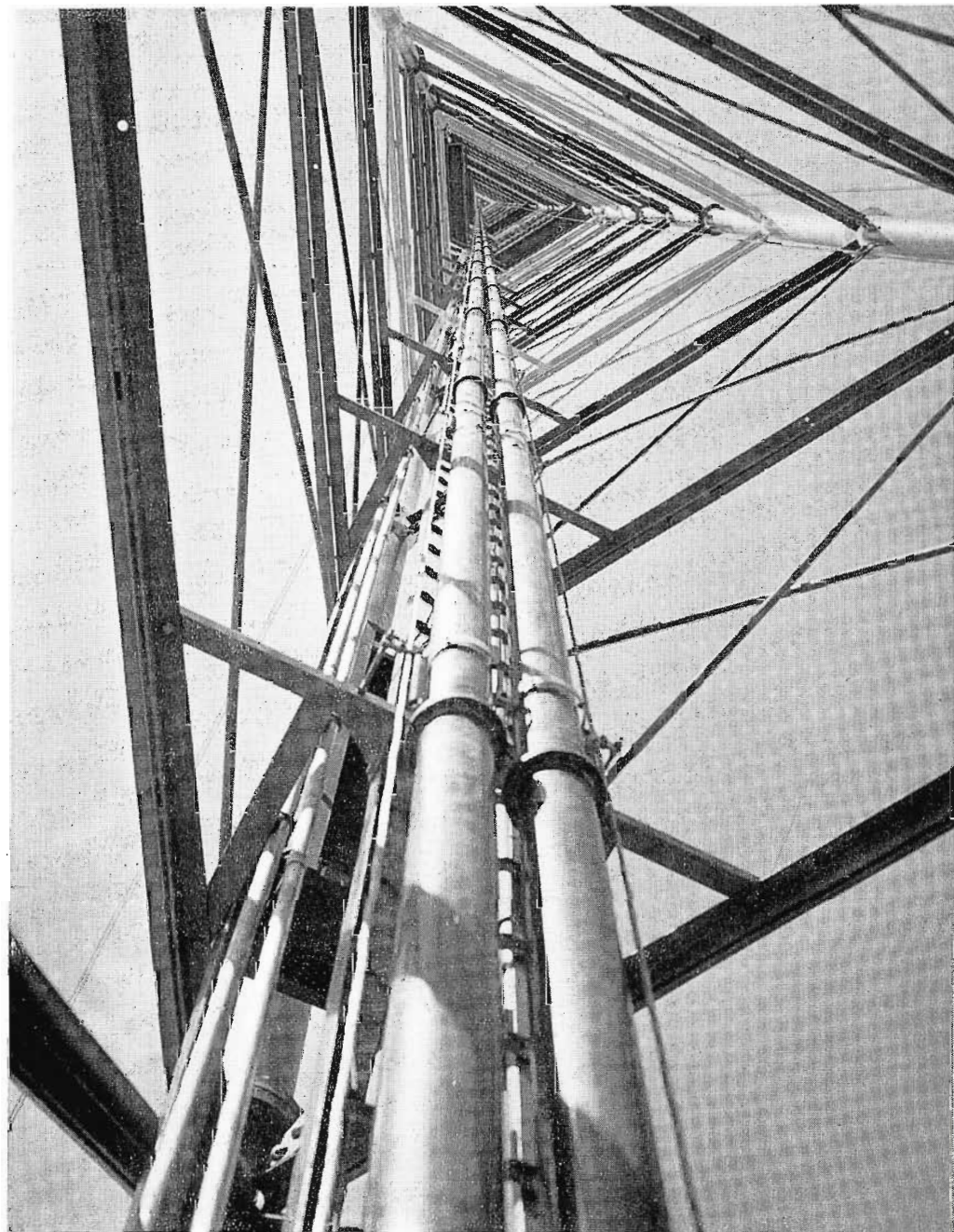
FIG. 7. Two 6 1/8" transmission lines—one for FM and one for TV—run up the inside of the tower. These lines are cable-supported, the method of anchoring being evident in this view.
