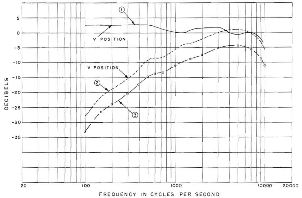
FIG. 6 (above). Measured response of the Type KB-3A "Close-Talk" Microphone.
