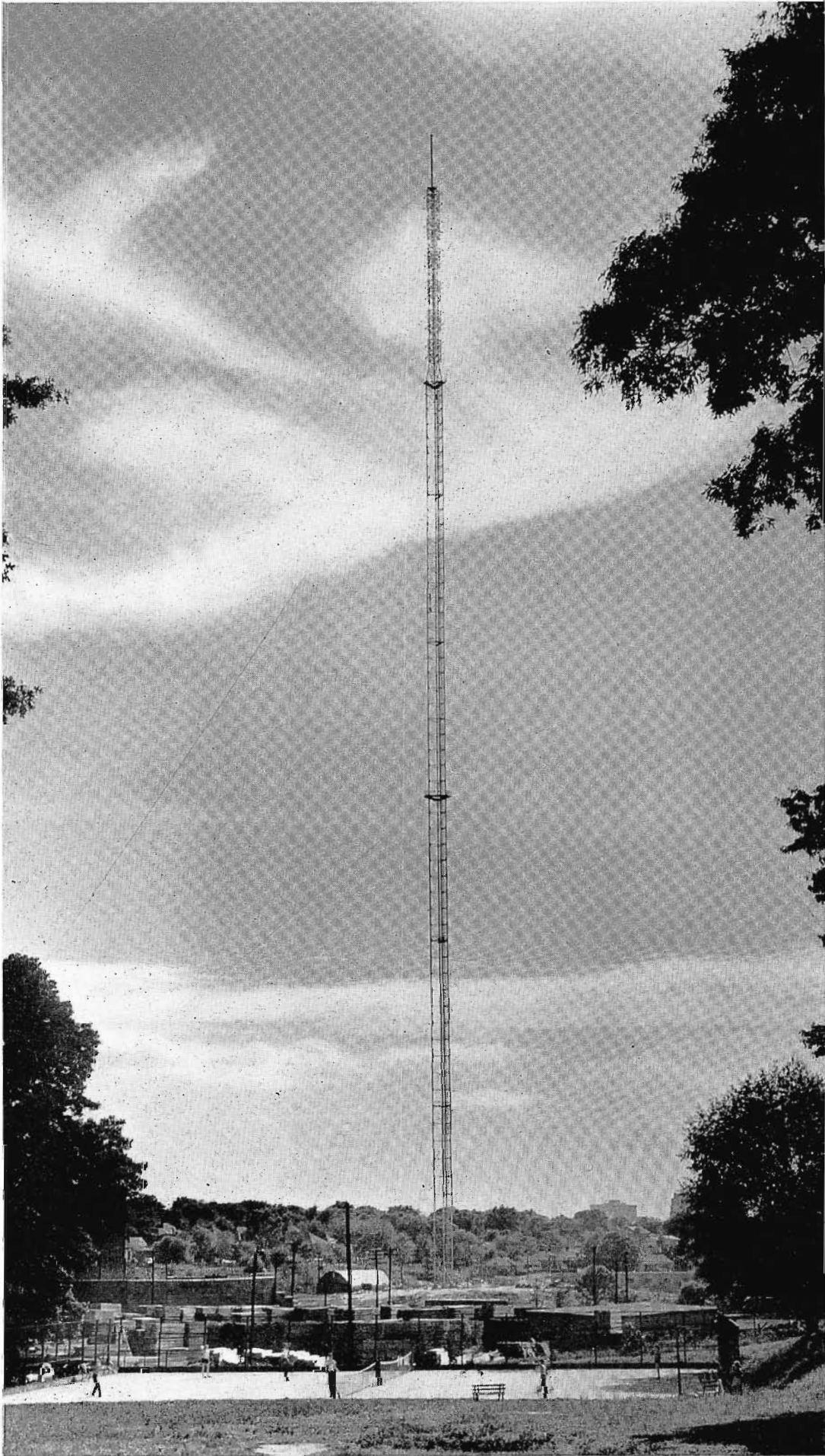
FIG. 1. View of the completed tower and antenna system from a point about a mile away. The location of the tower, in the very heart of Atlanta, provides high signal intensities in the city proper—while its tremendous height insures maximum coverage of surrounding areas.
