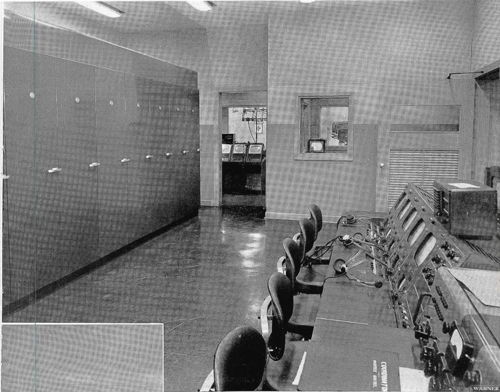
FIG. 4. View into WDAF-TV master control room where all switching operations take place. Small room (in front of camera) is the announce booth. Other small room to the left is a production booth, looking into studio.
