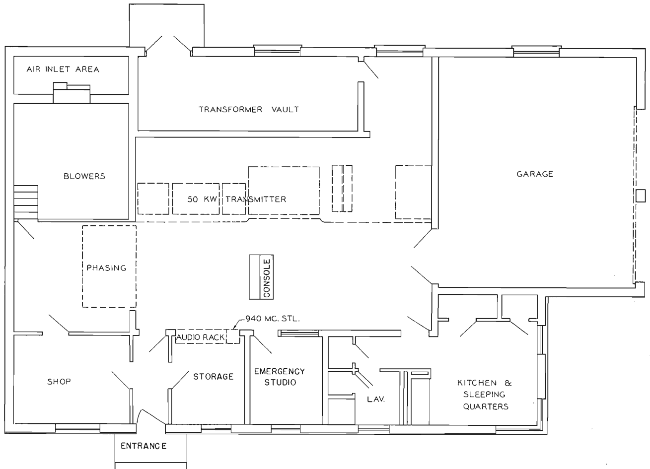
FIG. 2. Floor plan of the transmitter building which measures approximately 72 x 44 feet. Next to the storage room is an emergency studio which contains an auxiliary control panel with inputs to handle two microphones, two turntables, and the program circuit from the STL equipment. The studio building is located in downtown Tulsa, 18 miles away.
