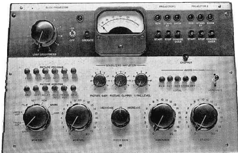
FIG. 2. Panel of TTC-3A1 Program Switching System. On this panel are controls for program levels, switches for audio-video selection and for remote control of two film projectors, plus a transmitter VU meter.
