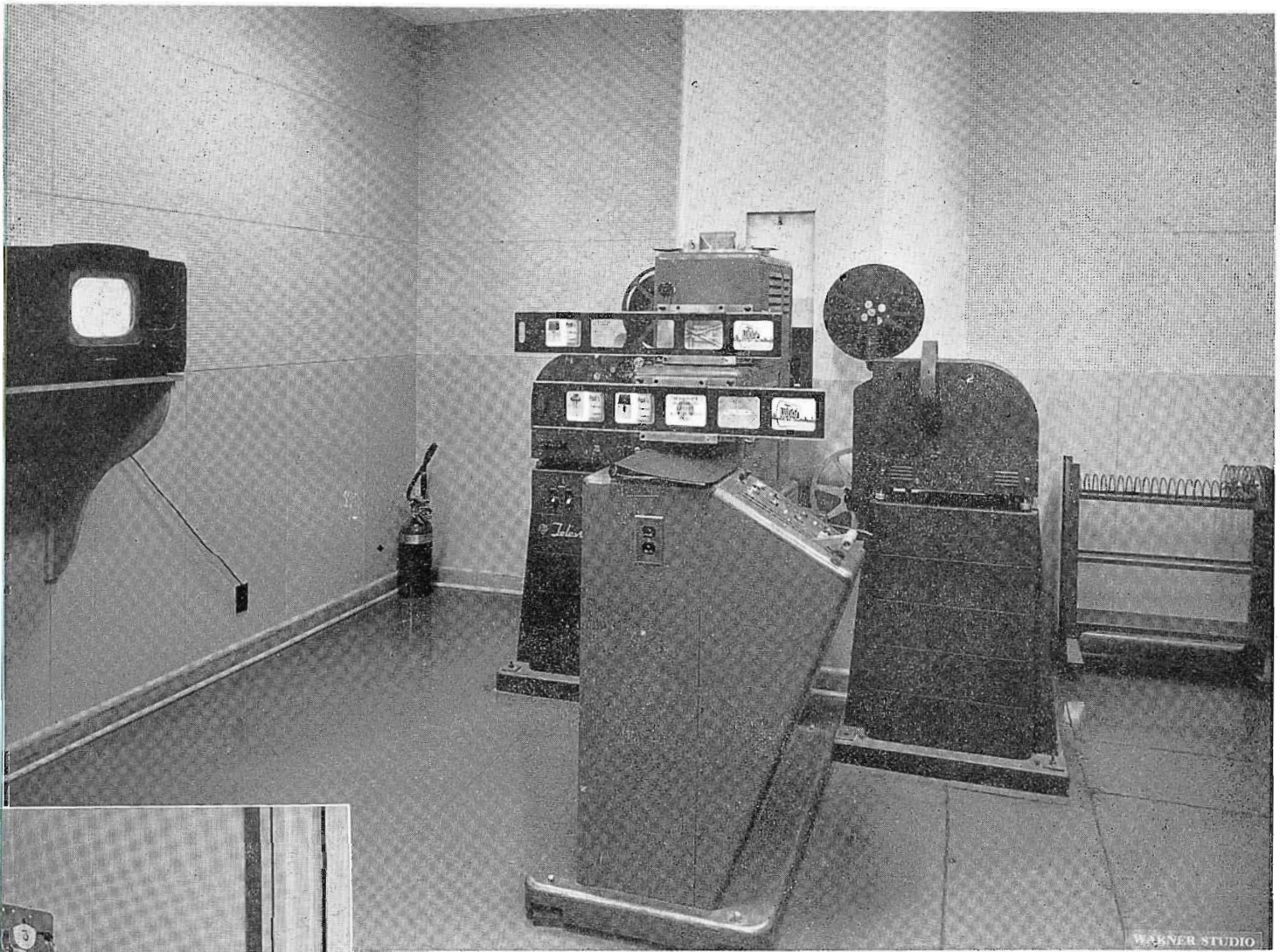
FIG. 7. WDAF-TV film projection room showing two 16mm projectors and the Gray Telop for transmitting the opaque slides. An RCA receiver is used as a line monitor. Note covered floor-trenches which carry all wiring for the projection equipment. These trenches were installed in many parts of the building, even to outside walls for future expansion.
