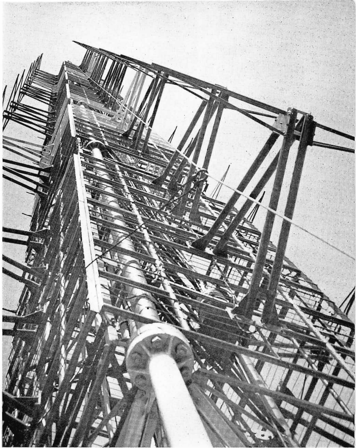
FIG. 4. Looking up at the RCA Supergain TV Antenna from the platform at the 800 foot point. Each radiating element is a reinforced dipole which is fed power by a concentric transmission line running through one of the slanting supporting numbers. The method of assembling the "bedspring" reflective shields in a four-sided arrangement (around the three-sided tower) is evident in this view.
