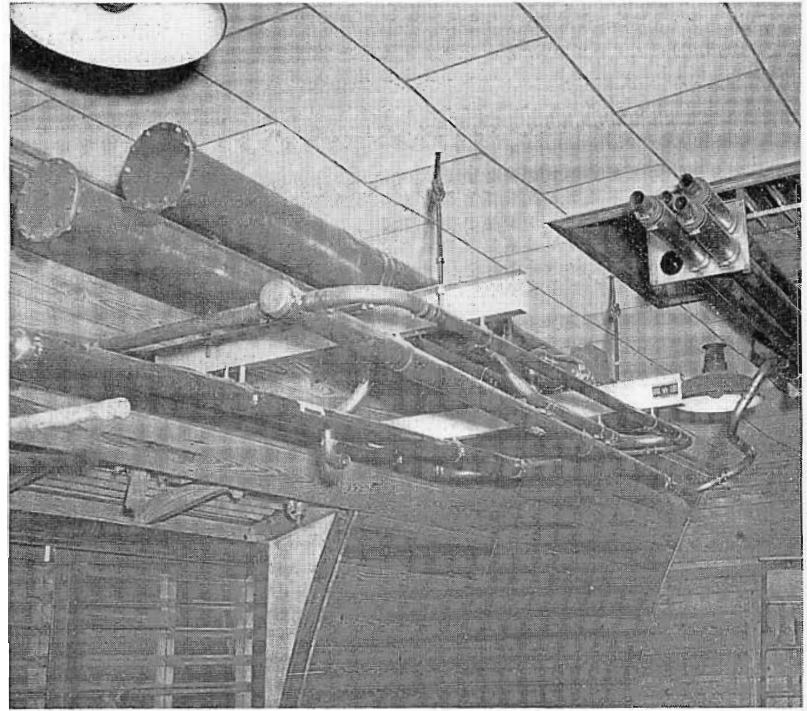
FIG. 12. The Notch Diplexer and Side-Band Filter in the TV transmission line are ceiling mounted units of the new simplified design.
