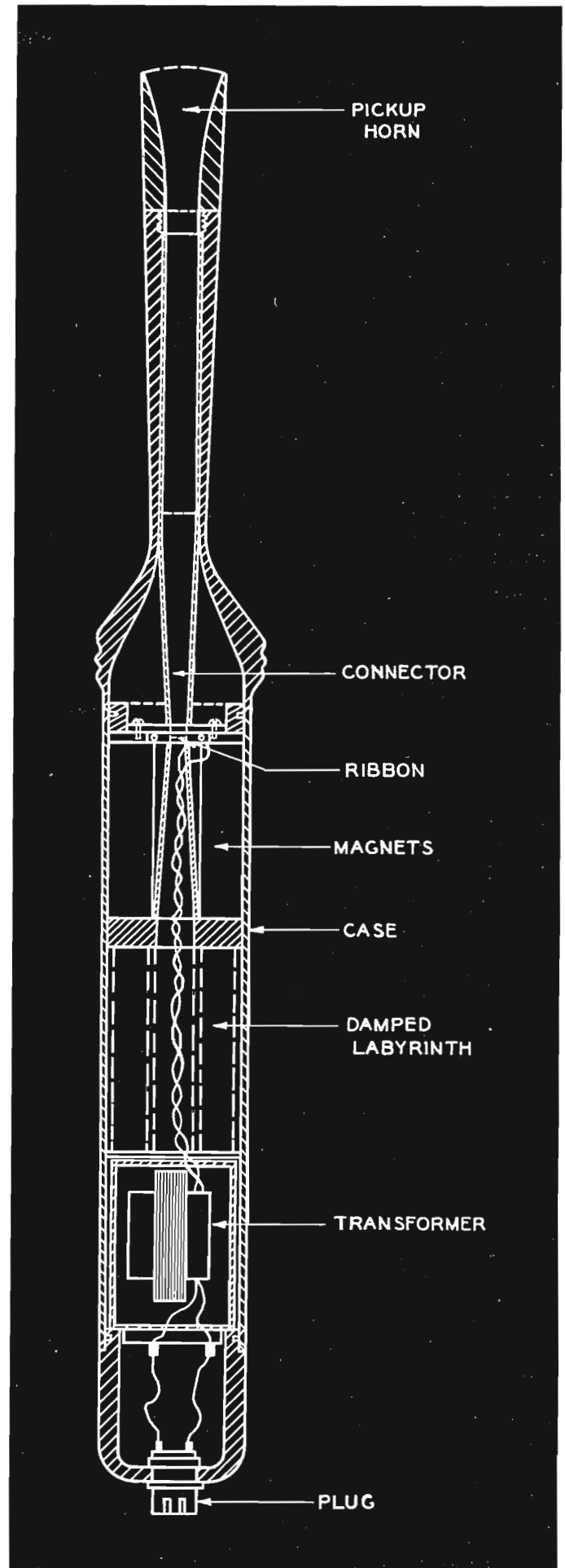
FIG. 6 (at right). This sectional view of the "Unobtrusive" Microphone illustrates the construction employed and shows how various parts are coupled together.
