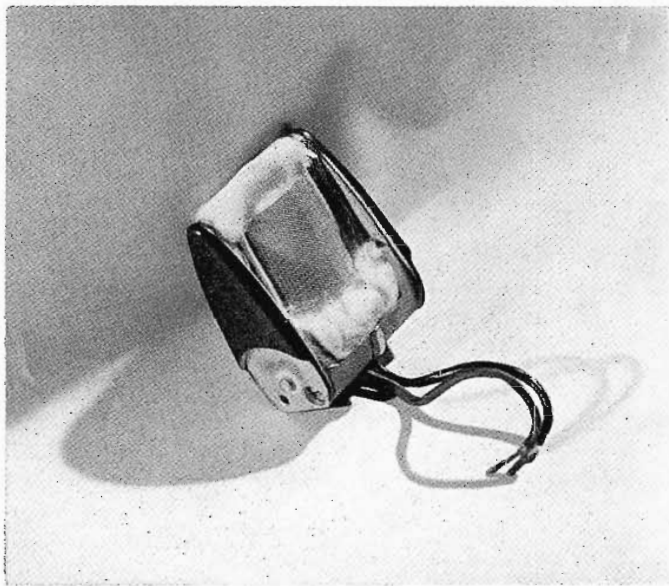
FIG. 4 (at left). View of the KB-3A Microphone with outer screen and part of the acoustical resistance (Fiberglass) removed to illustrate the inner (magnetic) screen. This screen prevents the entry of magnetic dirt particles into the microphone air gap.
