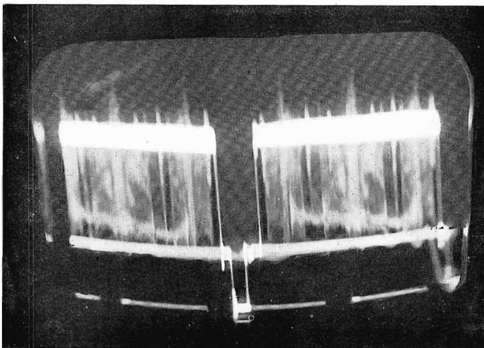
FIG. 1. The photograph from the monitor screen (at left) shows the waveform pattern as it would normally be seen when viewing the standard RMA video signal at the sweep frequency of 7,875 cycles (sawtooth). The diagram above identifies the various parts of the waveform in the photograph at the left. Explanation of the letter symbols is given in the text.
