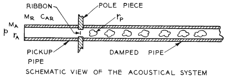
FIG. 2 (above). Acoustical system and circuit of a pressure type ribbon microphone. In the acoustical circuit: p = actuating sound pressure. M_A = inertance of the air load. M_R = inertance of the ribbon. C_{AR} = acoustical capacitance of the ribbon. r_A = acoustical resistance of the air load. r_P = acoustical resistance of the damped pipe. Z_{AE} = acoustical impedance due to the electrical circuit.
