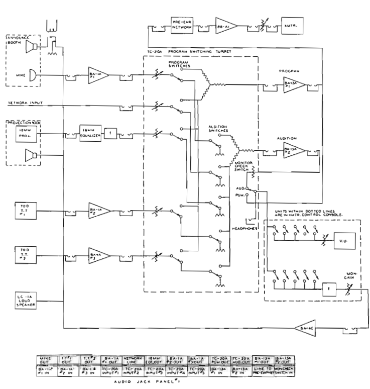
AUDIO FUNCTIONAL DIAGRAM
