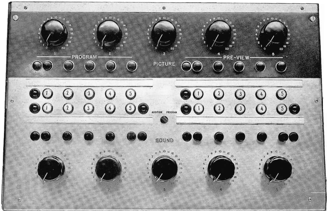
FIG. 9 (above). Panel view of MI-19063 Audio/Video Switching Turret. Capabilities of this system are shown by block diagram below. The system allows previewing and presetting of levels on as many as five audio and five video inputs. Turret is designed for use with standard transmitter consoles.
