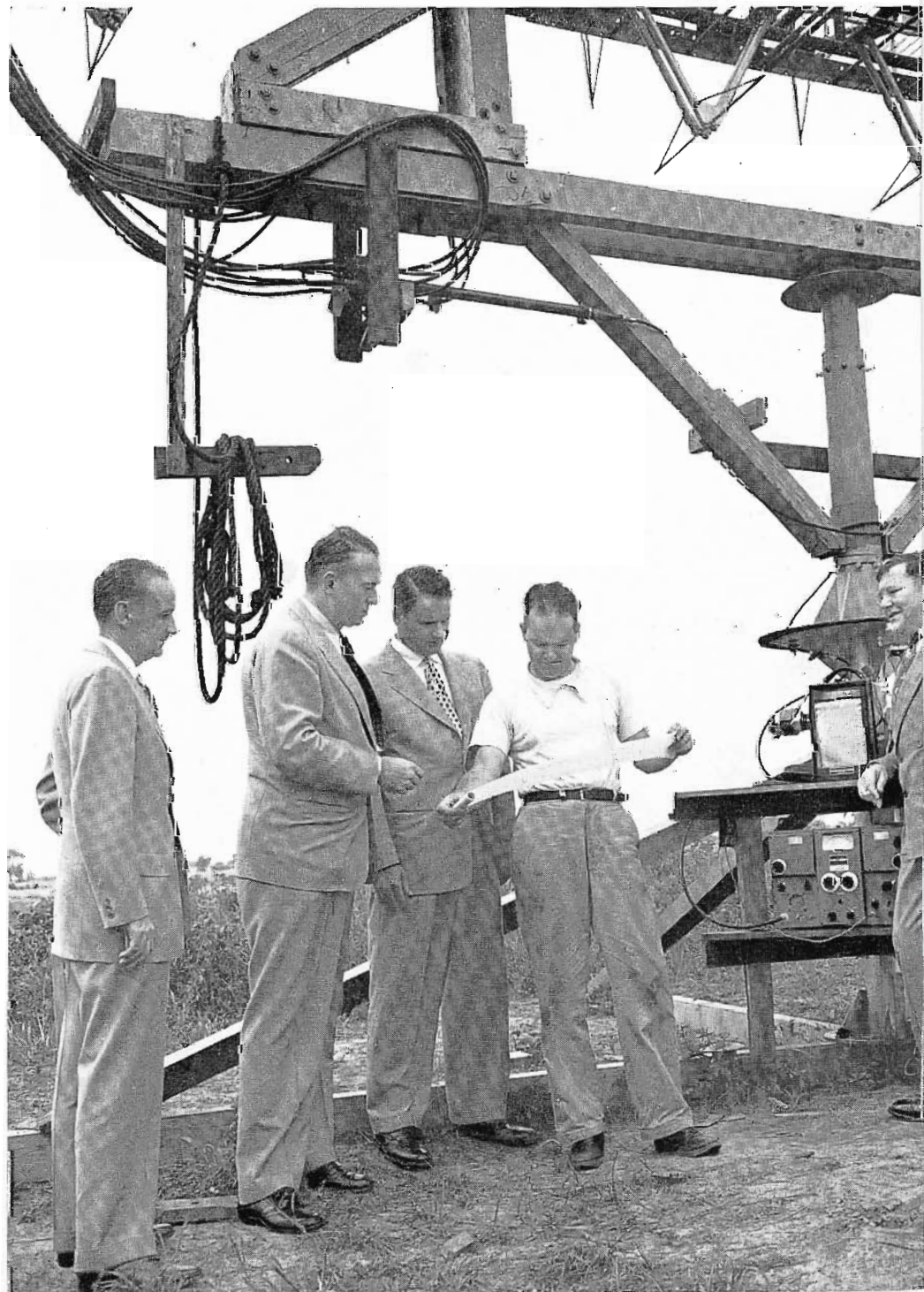
RIGHT: Closeup of the antenna measuring position. In making tests the antenna is used as a receiving antenna to pick up a signal from a fixed transmitter located a short distance away. Received signal is measured by field intensity meter at lower right and recorded on the Esterline-Angus Recorder as the antenna is rotated. Vertical radiation pattern is determined by this method. To determine horizontal pattern the antenna structure is mounted vertically and rotated about the vertical axis. Shown here discussing the operation are (left to right): Tom Howard, Chief Engineer of WPIX, one of the participating stations; Dr. F. G. Kear, of Kear and Kennedy, Consulting Engineers; C. W. Lyon, Jr., Executive Vice President of Empire State; R. S. Grimm, RCA Engineer; and E. S. Clammer, Manager of RCA Antenna Equipment Sales.
