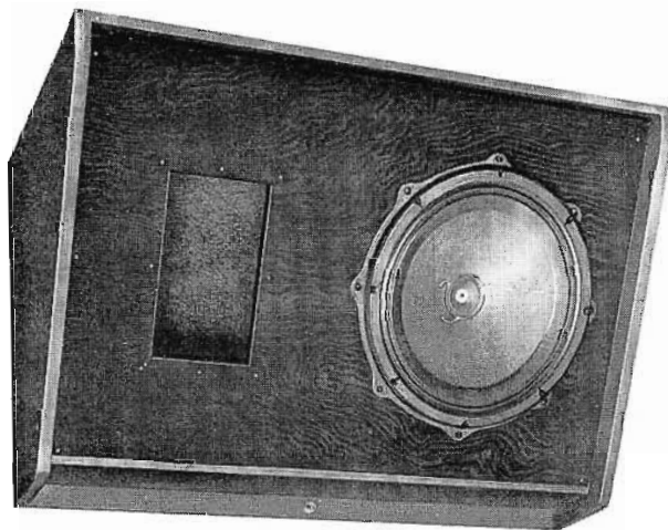
LC-5A HOUSING WITH DUO-CONE SPEAKER
