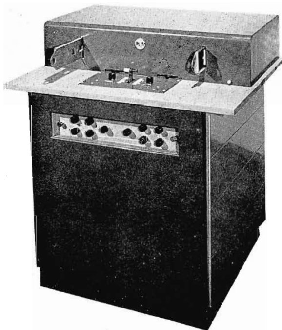
CONSOLE TYPE CABINET houses the complete Flying Spot Scanner and the variable masking arrangement used in obtaining video effects. (Additional circuits of the video effects equipment are mounted in a rack unit which may be located some distance away.) Two slide holders (each holding six slides) may be seen projecting from the upper case at convenient table level. Between them are located fading and lap dissolve controls. The operator can handle all operations from a comfortable sitting position.
