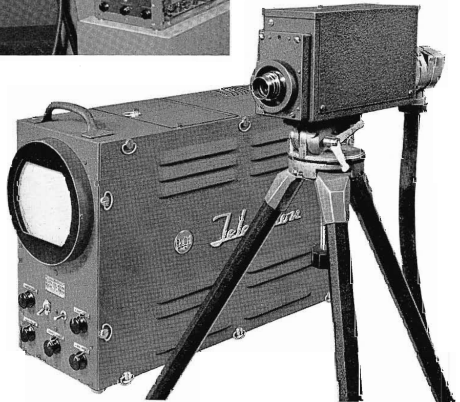
VIDECON EQUIPMENT is complete in these two units. The camera proper is only a little larger than a 16mm movie camera. The control unit which contains the sync generator, deflecting circuits, video amplifiers, controls and monitor kinescope is the same size as one of RCA's standard field units.
