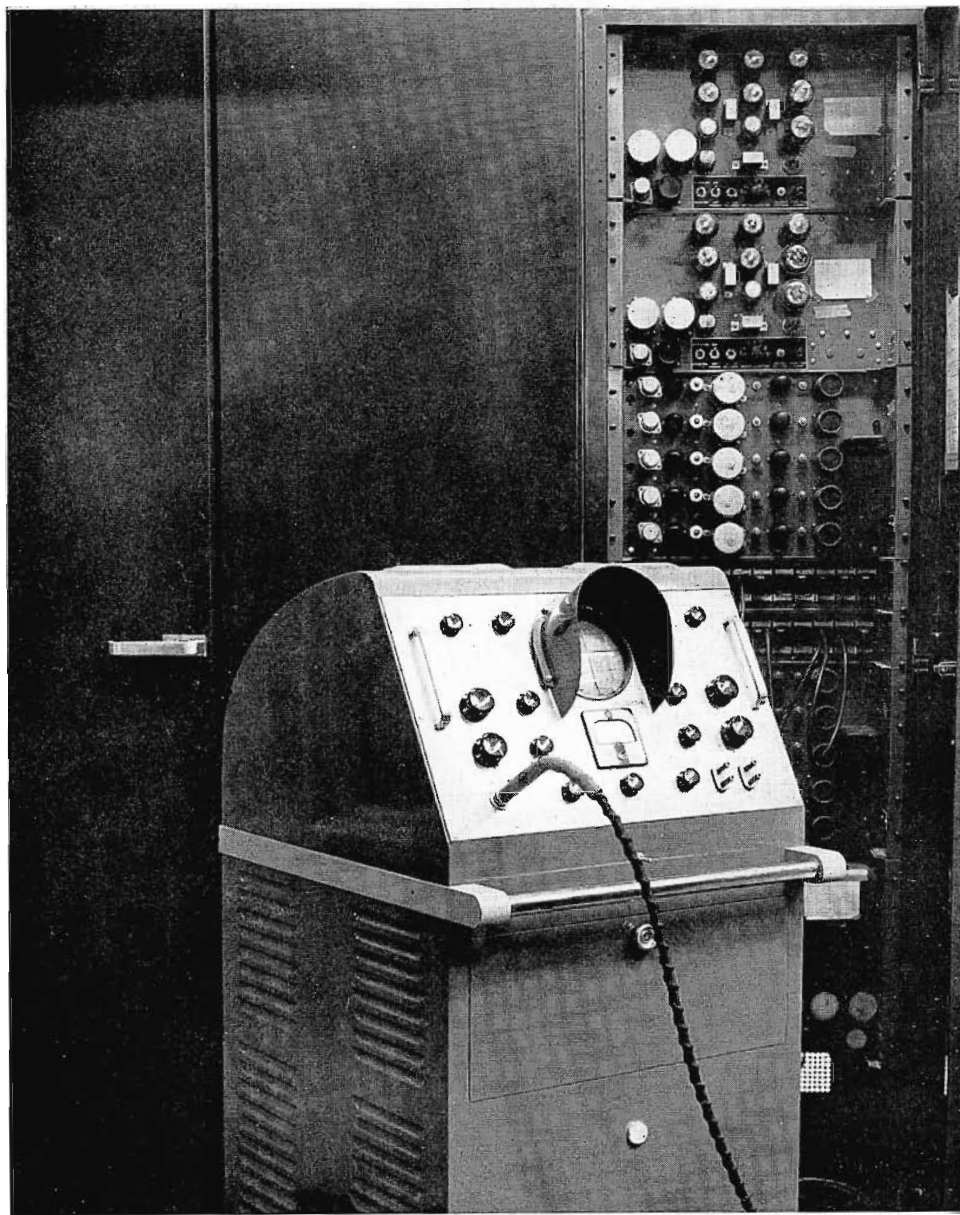
FIG. 3. In order to accurately reproduce these waveforms the oscilloscope used must have a response of at least ten times the horizontal pulse frequency. Either the regular monitor scope (which has a response 300 times the pulse frequency) or an RCA 715-B Oscilloscope, such as that shown here, may be used.
