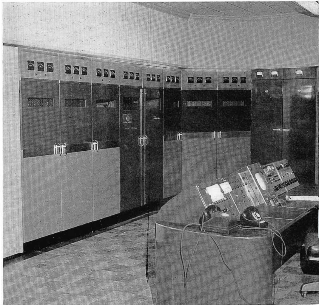
FIG. 10 (above). The 10 KW RCA FM Transmitter and the 5 KW RCA TV Transmitter are arranged in line with the left and right ends, respectively, bent around so that the equipment units form a shallow U. In the center of the U is the combined control desk. The view above shows the control desk and left side of the FM transmitter.
