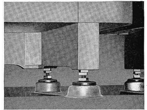
FIG. 1 (above). Partial closeup of 70-C2 turntable legs showing how "Lord" shock mounts are employed.
